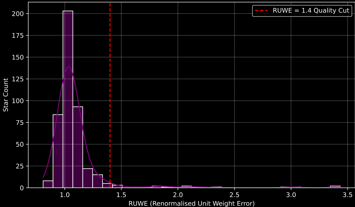
GAPOGEE DR17 Field [210-04] RUWE Distribution (n= 447)
