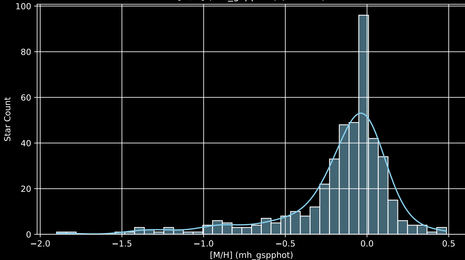
APOGEE DR17 Field: [210-04 [M/H] (mh_gspphot) (n= 449)
