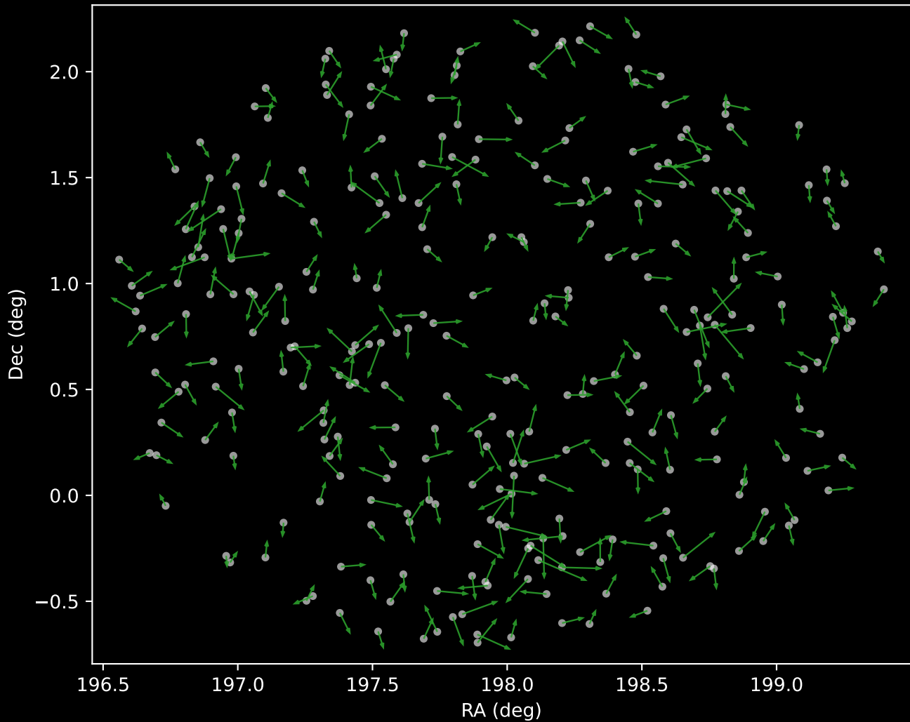
APOGEE DR17 Cluster 4 Proper Motion Vectors (n=296)
