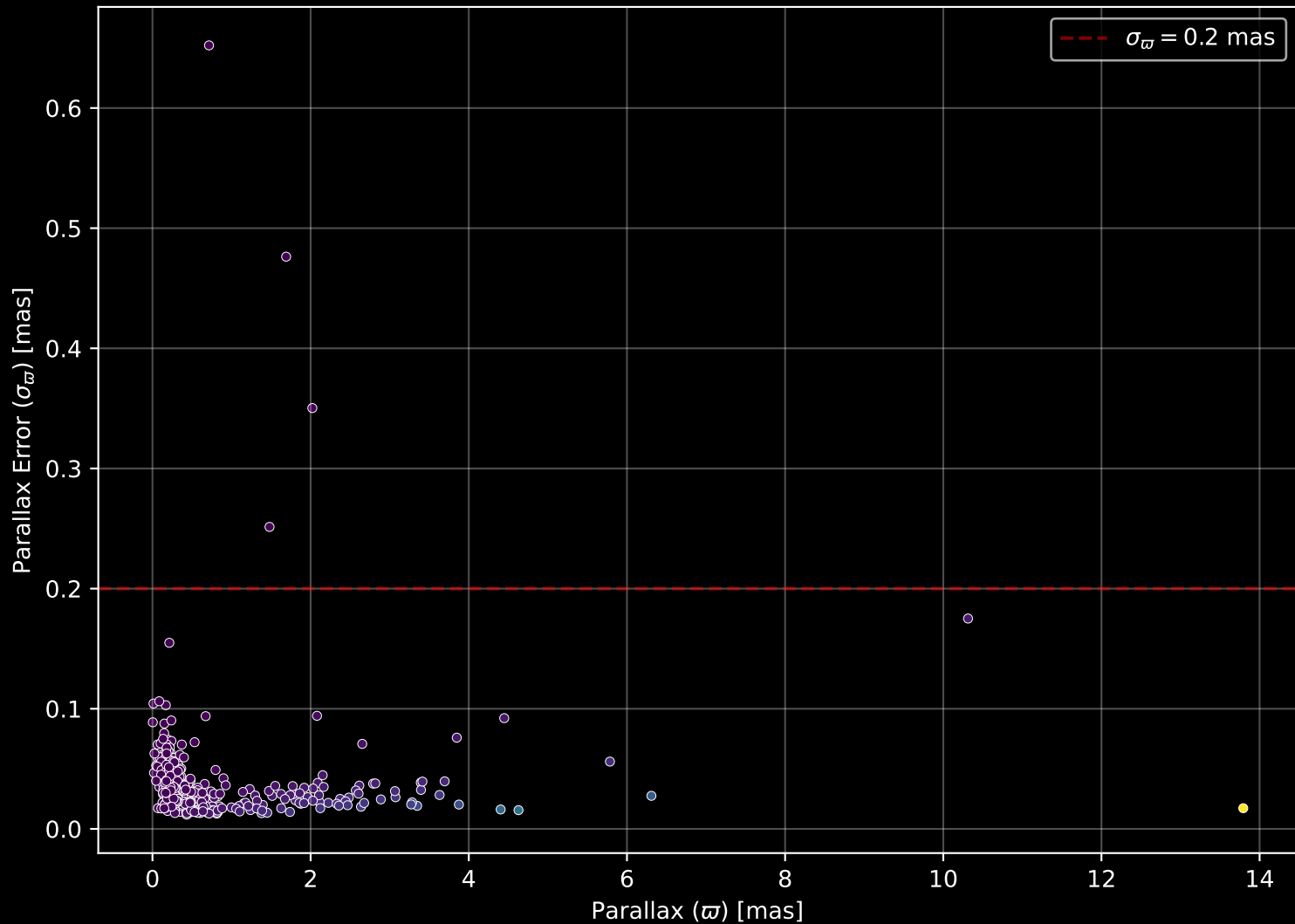
APOGEE DR17 Field: [210-04] Parallax Quality (n= 452)
