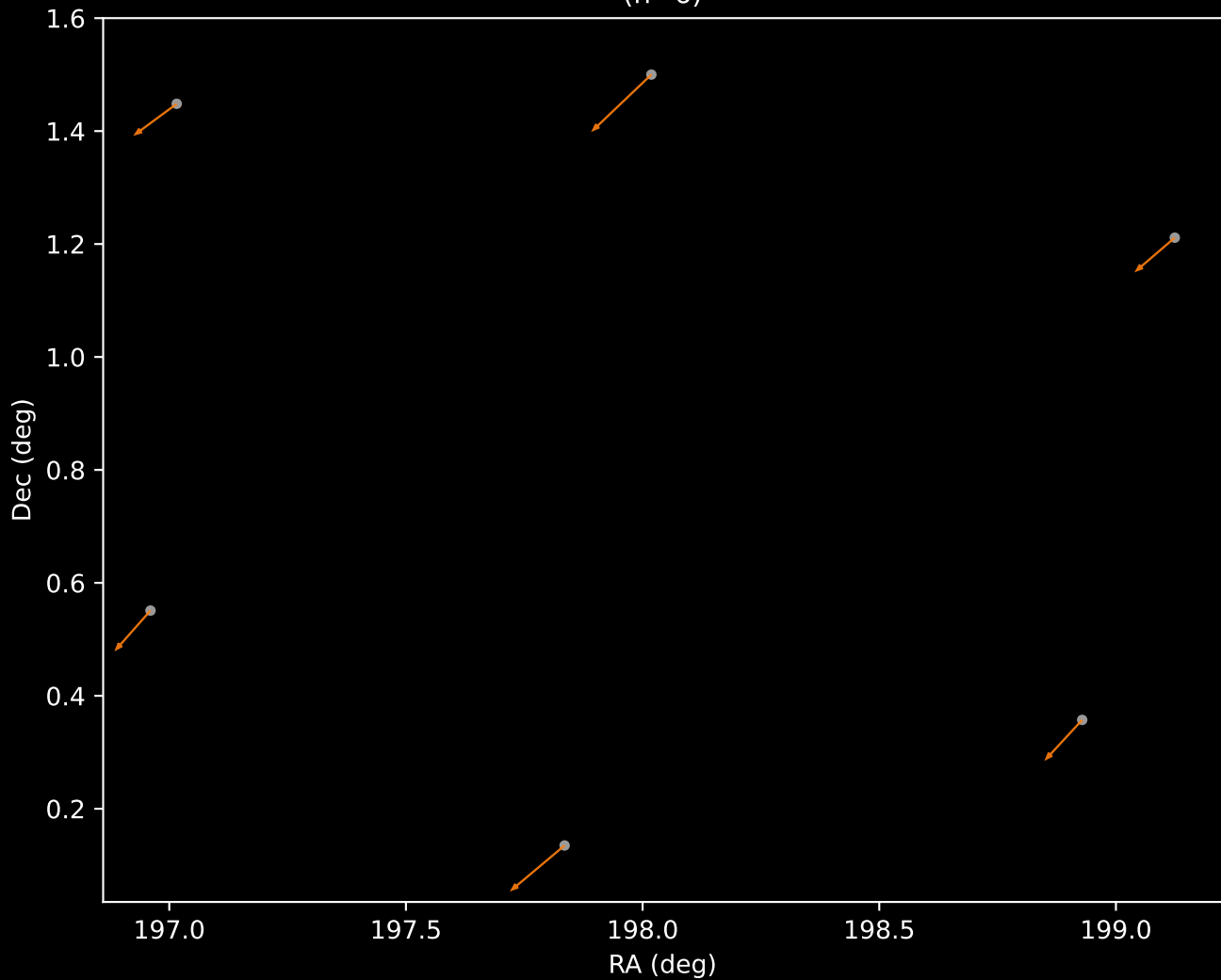
APOGEE DR17 Cluster 2 Proper Motion Vectors (n=6)
