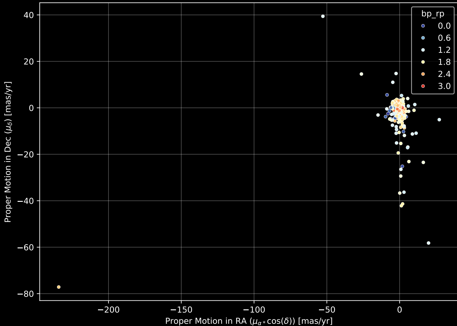
APOGEE DR17 Field: [210-04] Proper Motion Diagram (n= 452)
